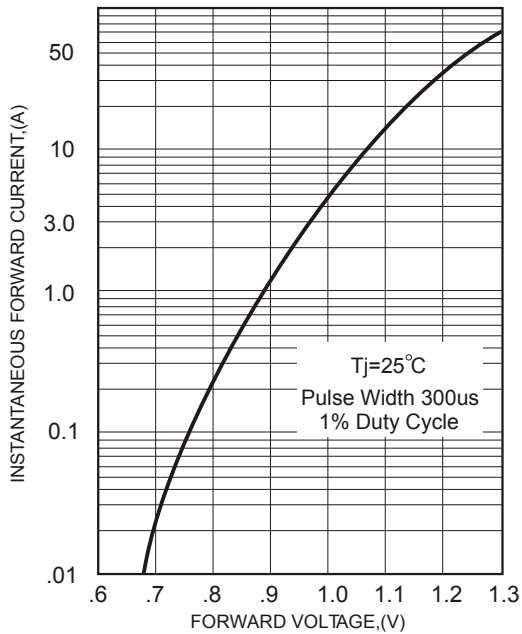
FIG.1-TYPICAL FORWARD CHARACTERISTICS
